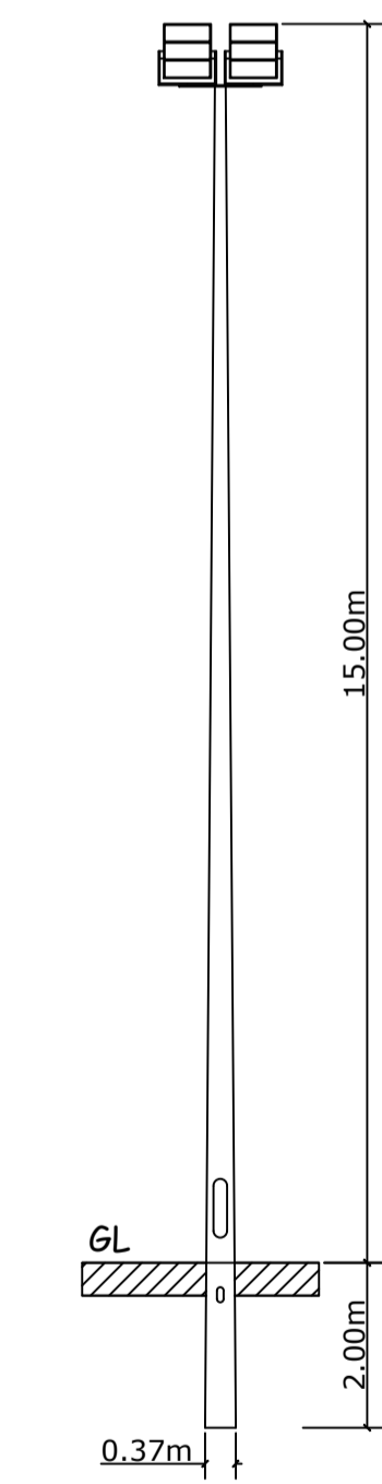
15m High Floodlight Pole Scale: 1:100
