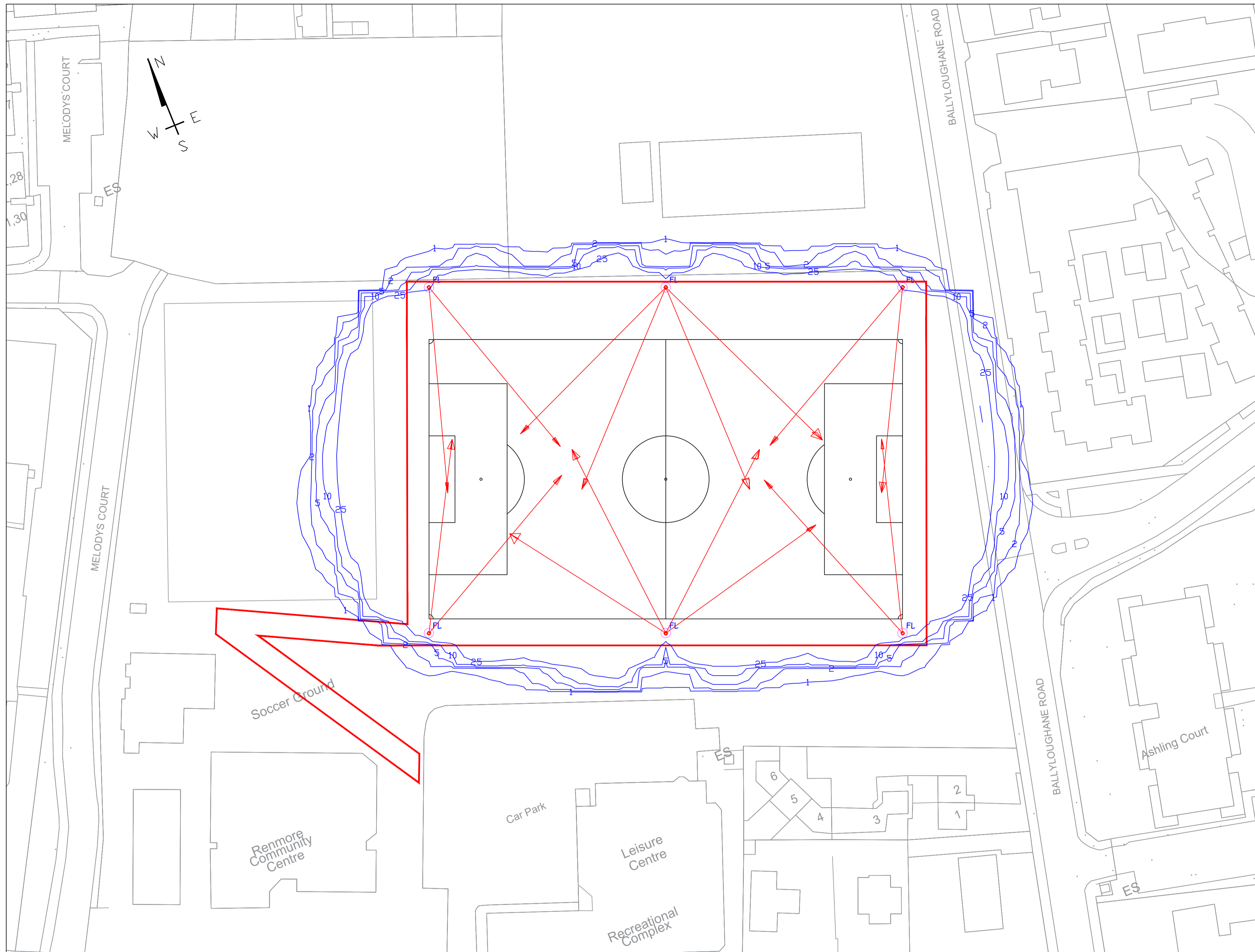
Pitch Lighting - Overspill Iso Contours Scale 1:500
