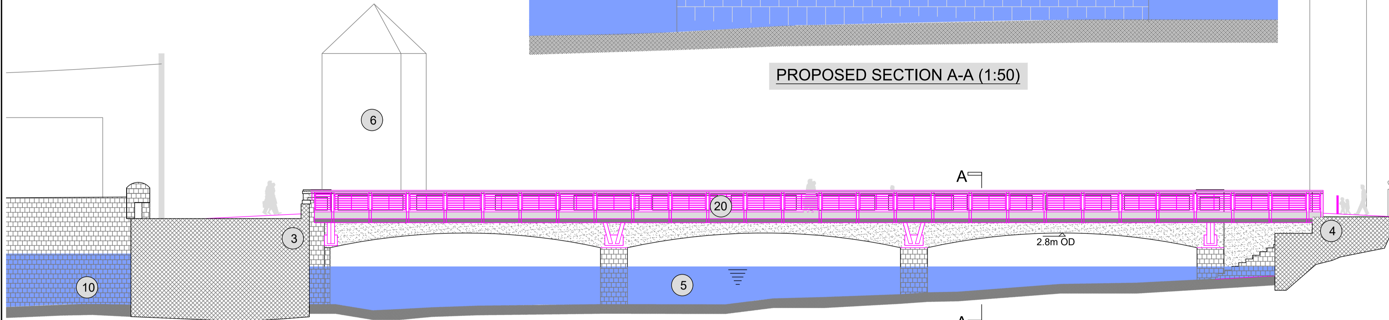
PROPOSED DOWNSTREAM ELEVATION (1:125)
