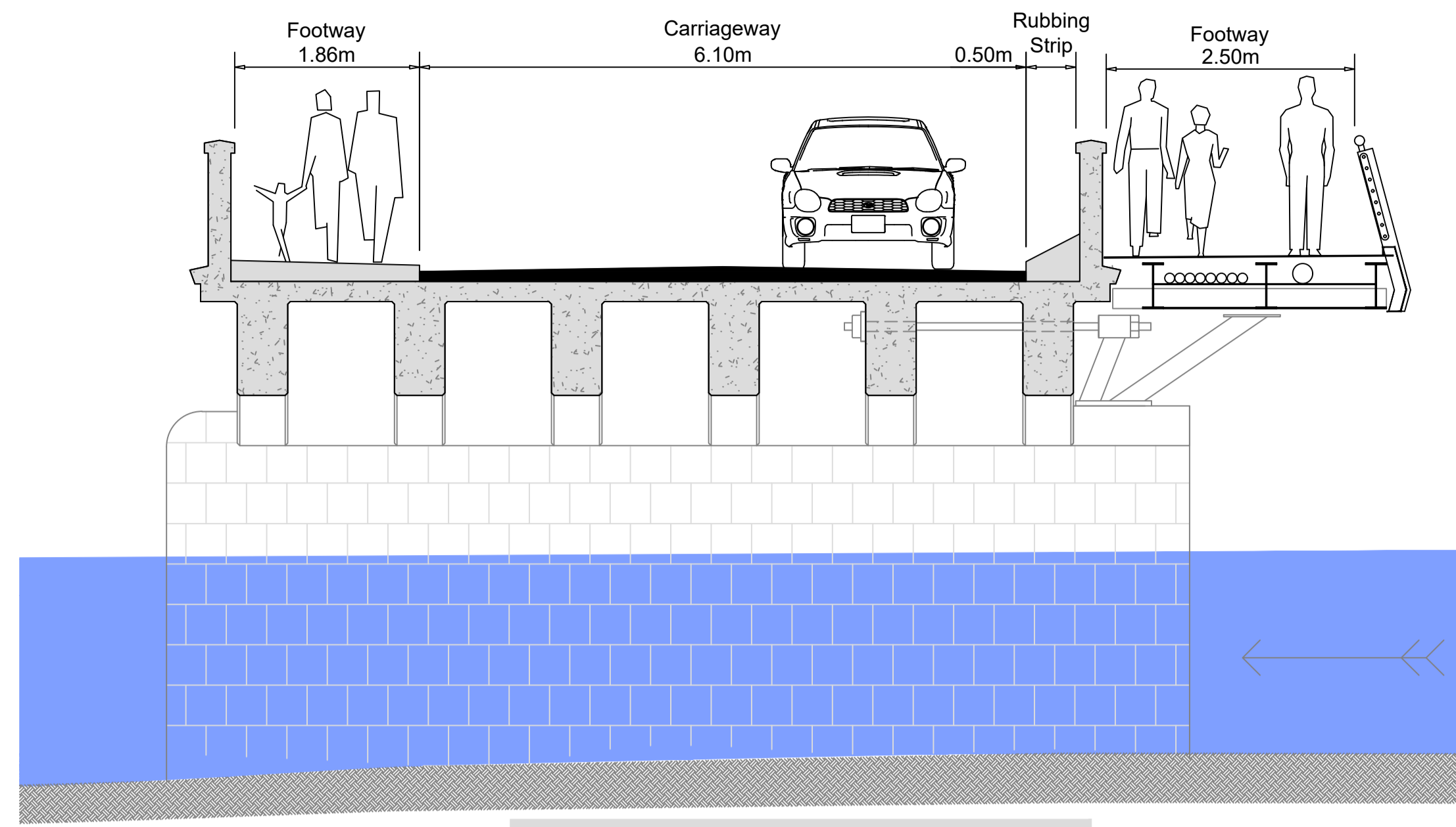
EXISTING CROSS SECTION (1:50)
