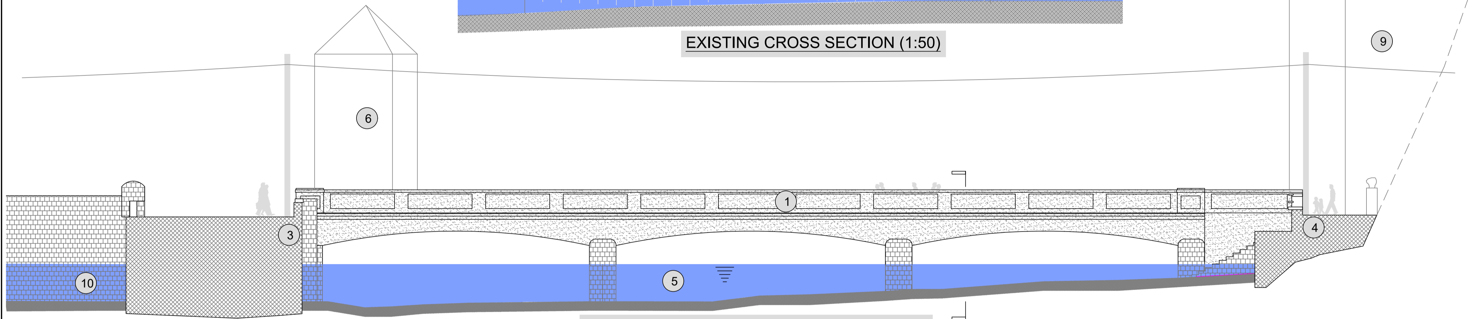
EXISTING DOWNSTREAM ELEVATION (1:125)
