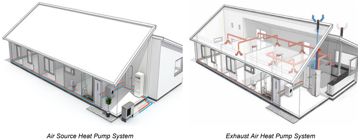
Air Source Heat Pump System
